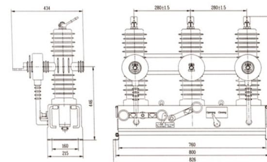
Figure 1 Smart switch body outline drawing
