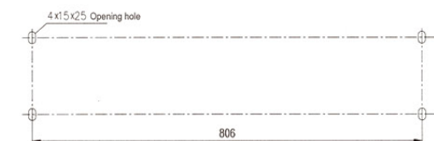
Figure 2 Smart switch body outline drawing
