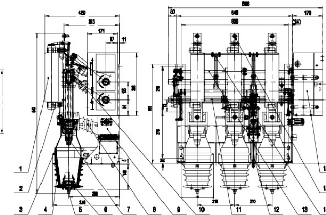
FKRN12A-12D Dimension of air-pressure load switch-fuse combination with right operation (inversion)
