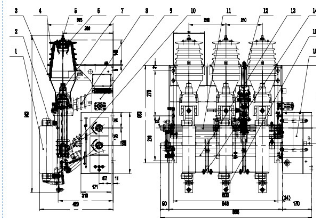
FKRN12A-12D Dimension of air-pressure load switch-fuse combination with right operation
