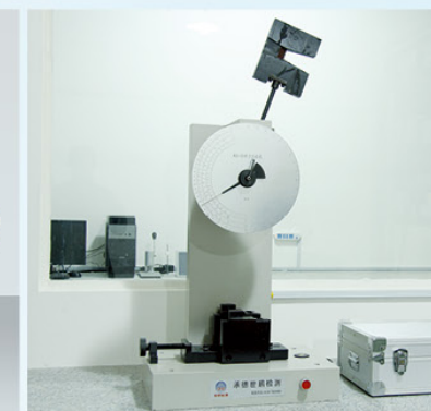
Impulse strength testing machine
